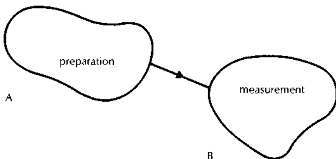
observation of a particle in atomic physics
