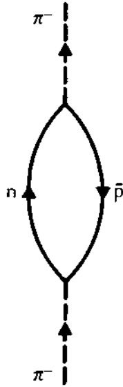
creation of a virtual neutron-antiproton pair
