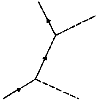
electron-photon scattering
