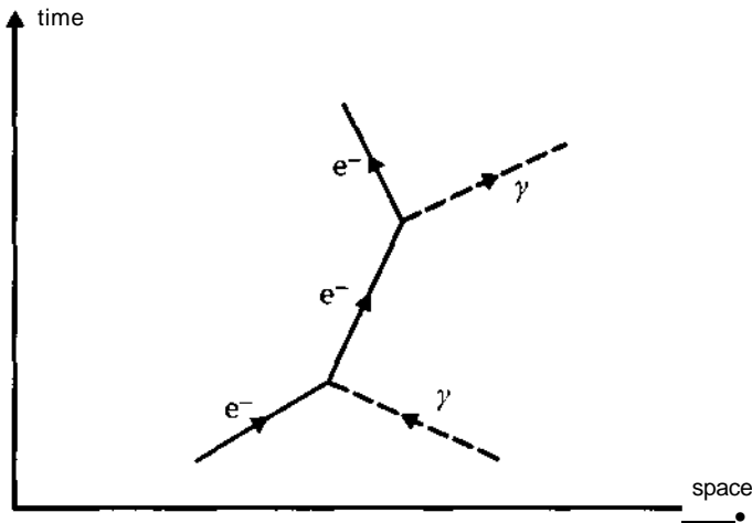
electron-photon scattering
