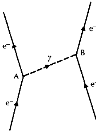
mutual repulsion of two electrons through the exchange of a photon
