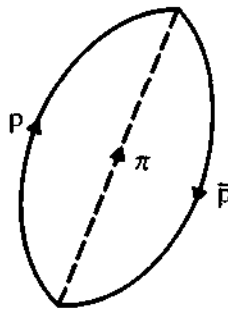
a vacuum diagram
