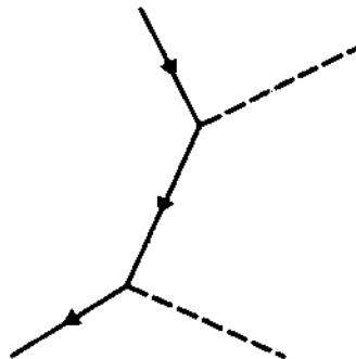
positron-photon scattering
