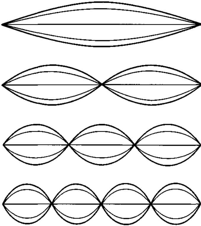
standing-wave patterns in a vibrating string
