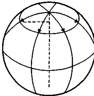
drawing a circle on a sphere
