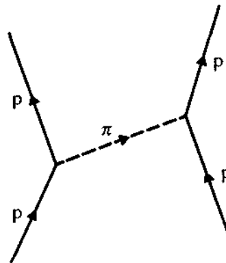
exchange of a pion ( n ) between two protons ( p )
