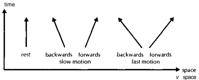
world lines of particles
