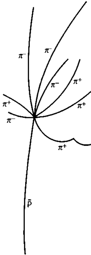
Creation of eight pions in a collision between an antiproton ( \bar{p} ) and a proton (sitting in the bubble chamber); see photograph on preceding page
