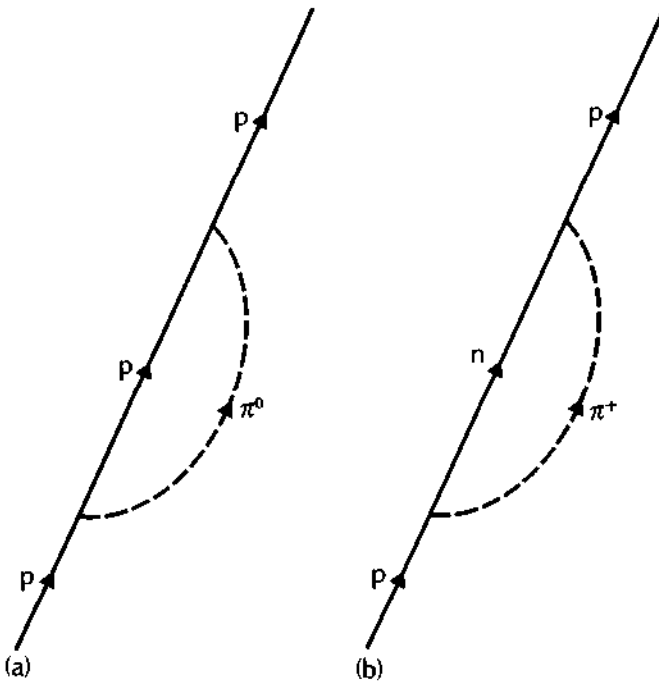
Feynman diagrams showing a proton emitting and reabsorbing virtual pions
