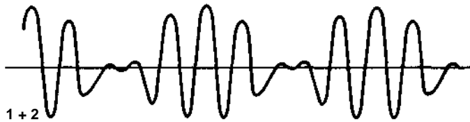
interference of two waves
